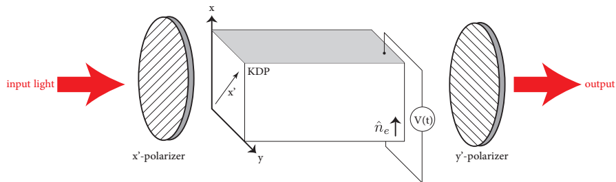
Figure : a transverse optical modulator
